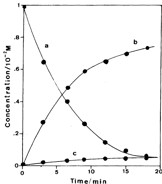
Fig. 2. Concentration vs. time curve for the PNO-catalyzed two-phase reaction of PhCOCl and o -C 6 H 4 (COONa) 2 (Type 2); [ o -C 6 H 4 (COONa) 2 ] i,aq = 0.500 M, [PNO] i,aq = 6.00 × 10 -4 M, [PhCOCl] i,org = 0.0100 M, 18 °C. a: PhCOCl, b: o -C 6 H 4 -(COOCOPh)(COOH), c: (PhCO) 2 O (corrected). [(PhCO) 2 O] corrected = 2 × [(PhCO) 2 O] org .
